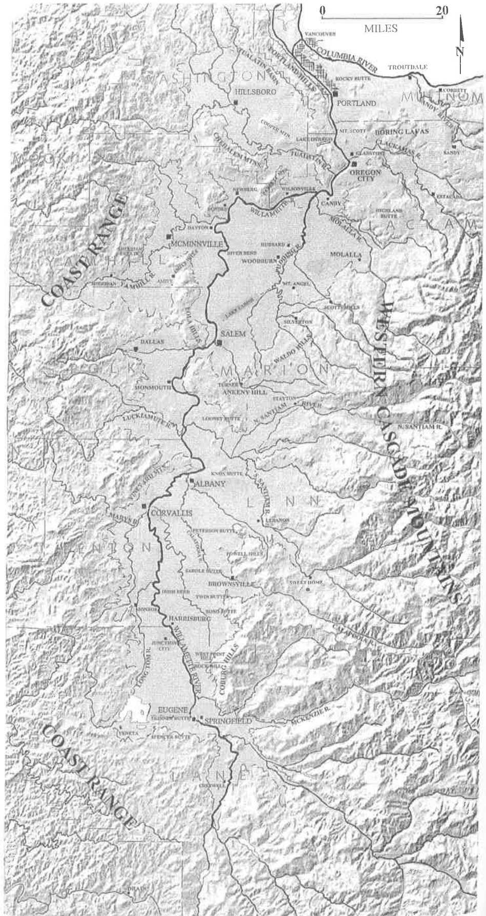
Physiographic map (After Loy, et al., eds., 2001)
