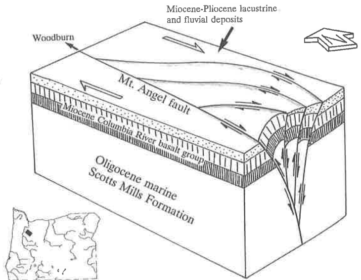
The butte at Mt. Angel, where the Abbey sits, forms what is called a fault "pop-up" in which rocks, caught and squeezed between a series of intersecting fault blocks, are slowly extruded to the surface. (After Werner, et al., 1992)
