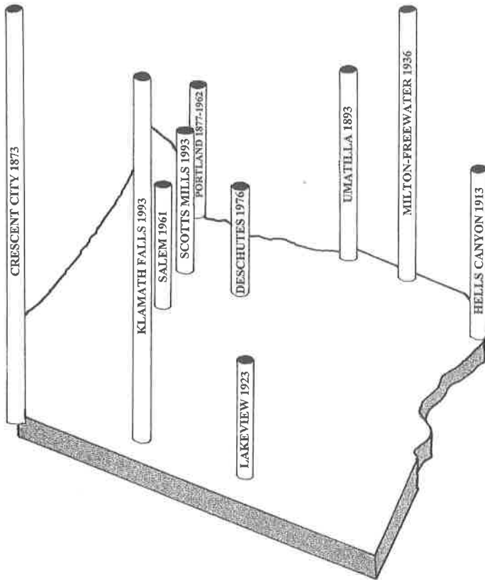
A look at large earthquakes in Oregon shows most measured VI on the Mercalli scale. Only the Crescent City (California), Klamath Falls, Milton-Freewater, and Portland quakes were stronger at VII. (After Berg and Baker, 1963; Byerly, 1952; Madin and Mabey, 1996; Niewendorp and Neuhaus, 2003; Townley and Allen, 1939; Wong and Bott, 1995)
