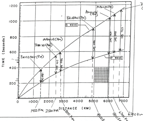
Figure IV-11 Travel-Time Curves for P and S Waves
