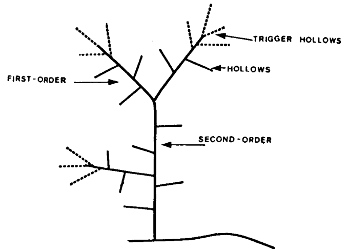
FIG. 2. Hypothetical channel network showing the location of trigger hollows.
