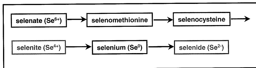
FIGURE 5 Decreasing order of bioavailability of the different forms of selenium found in soils.
