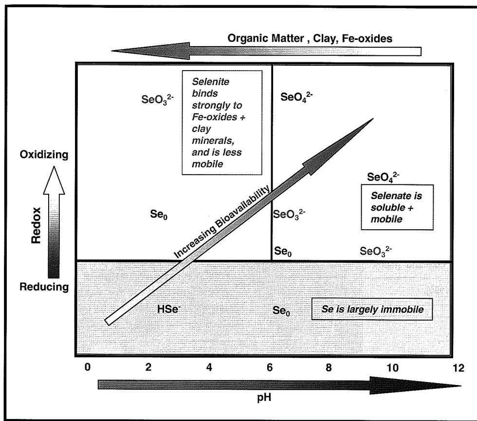
FIGURE 4 Schematic diagram showing the main controls on the chemical speciation and bioavailability of selenium in soils.
