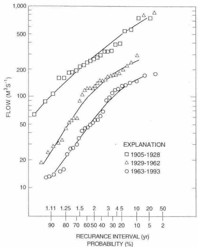
Figure 2. Reductions in flood regime induced by reservoirs, illustrated by flood frequency analysis for the Mokelumne River below the Camanche Dam (U. S. Geological Survey gauge No. 11323500), for three time periods: before the Pardee Dam (1905–1928), after the Pardee Dam but before the Camanche Dam (1929–1962), and after the Camanche Dam (1963–1993). Mean annual runoff is 932 \times 10^6 \text{ m}^3 ; Pardee impounds 259 \times 10^6 \text{ m}^3 (28% of annual runoff); and Camanche 532 \times 10^6 \text{ m}^3 (54% of annual runoff). (Source of data: U.S. Geological Survey published data, California Department of Water Resources 1984).
