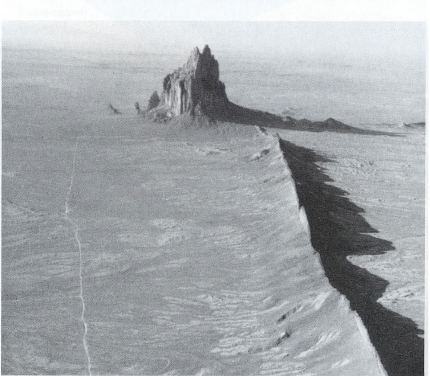
FIGURE 11-31 Volcanic neck with radial dike, Shiprock, New Mexico.
