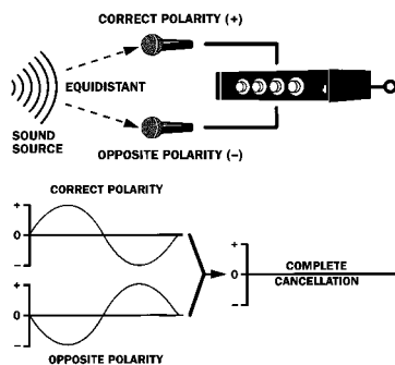
Polarity reversal
